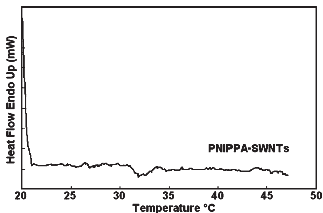
Figure 8. DSC curve of PNIPPA-SWNTs in water
