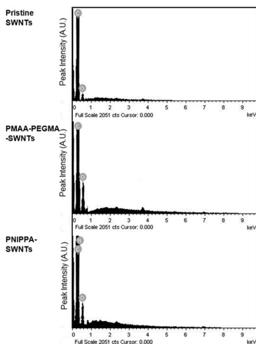
Figure 3. Survey EDS spectra of pristine SWNTs, PMAA-PEGMA-SWNTs, and PNIPPA-SWNTs.
