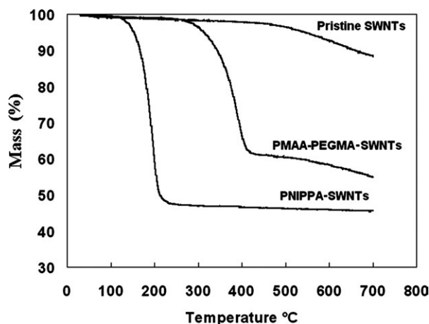
Figure 4. TGA curves of pristine SWNTs, PMAA-PEGMA-SWNTs, and PNIPPA-SWNTs.
