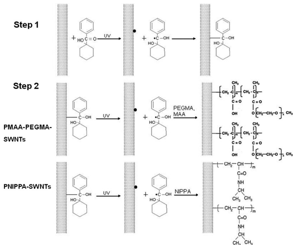
Scheme 1. Illustration of the fabrication of pH and temperature-responsive single wall carbon nanotubes.
