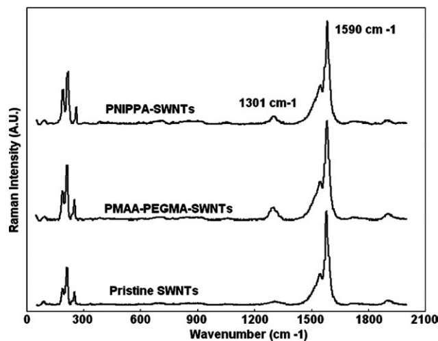
Figure 2. Raman spectra of pristine SWNTs, PMAA-PEGMA-SWNTs, and PNIPPA-SWNTs.
