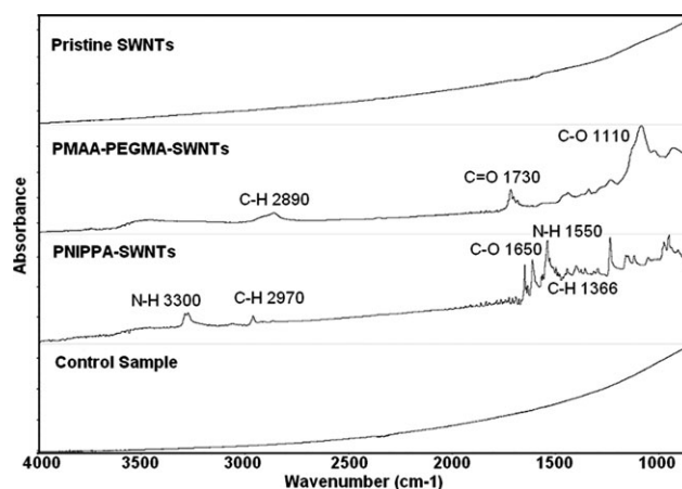
Figure 1. ATR-FTIR spectra of pristine SWNTs, PMAA-PEGMA-SWNTs, and PNIPPA-SWNTs.
