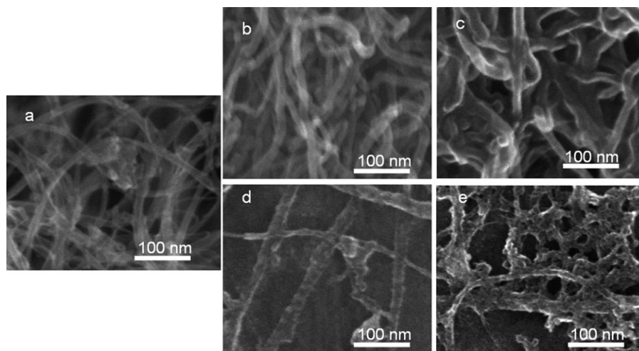
Figure 5. SEM images of (a) pristine SWNTs, (b) PMAA-PEGMA-SWNTs at pH 10, (c) PMAA-PEGMA-SWNTs at pH 4, (d) PNIPPA-SWNTs at room temperature, (e) PNIPPA-SWNTs at 35°C.
